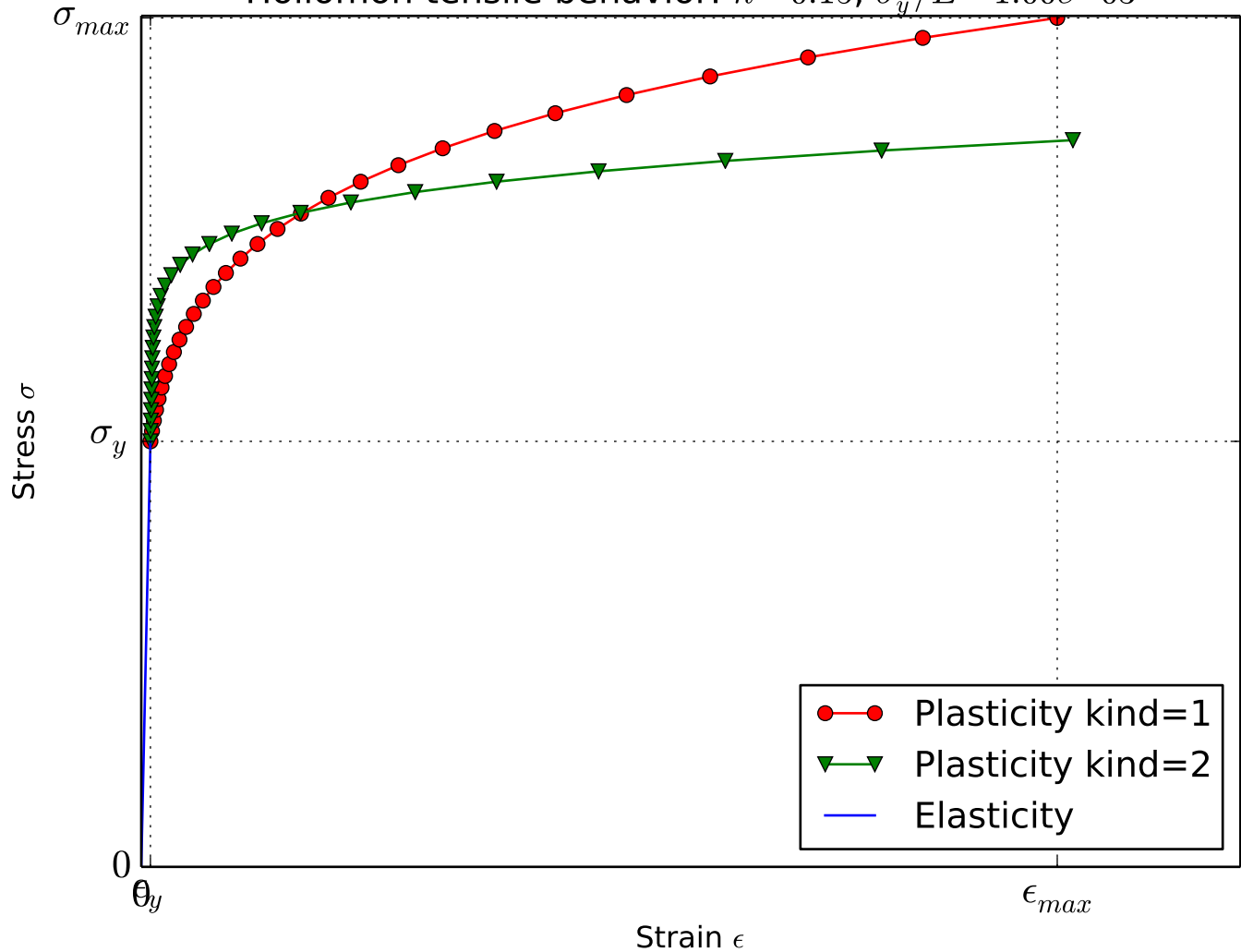
Hollomon tensile behavior: n = 0.15 , \sigma_y / E = 1.00e-03
